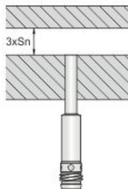
Flush mounting
